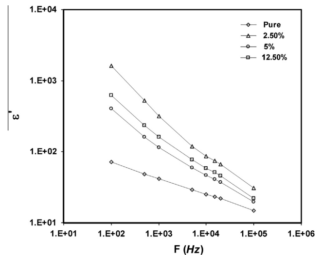
Fig. 6a Frequency dependence of dielectric constant \epsilon' for CuI/PVA polymer composite with different concentrations of CuI at 303 K.
